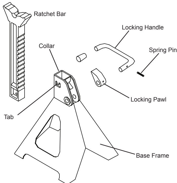
Figure 1 - 32035/32065 Jack Stand Components
