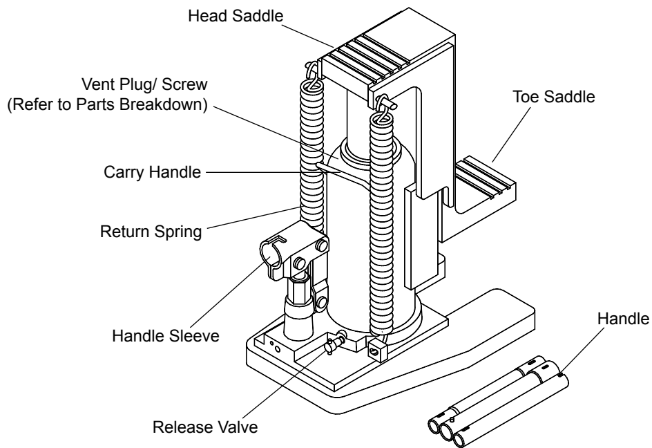
Figure 1 - 13060, 13120 & 13200 Nomenclature
