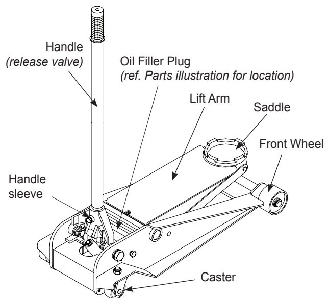
Figure 1 - Typical Jack Nomenclature
