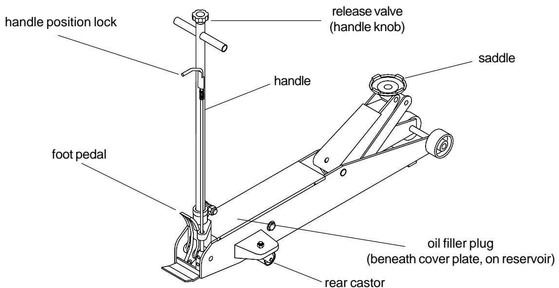
Figure 1 - Model 25048, 25058 & 25108 Nomenclature
