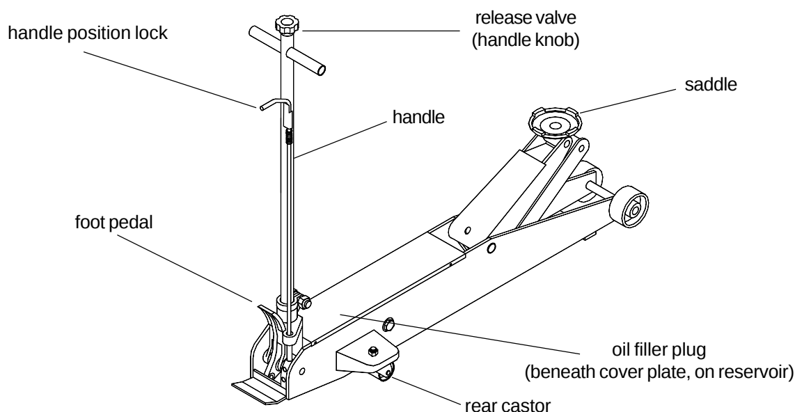
Figure 1 - Model 25048, 25058 & 25108 Nomenclature
