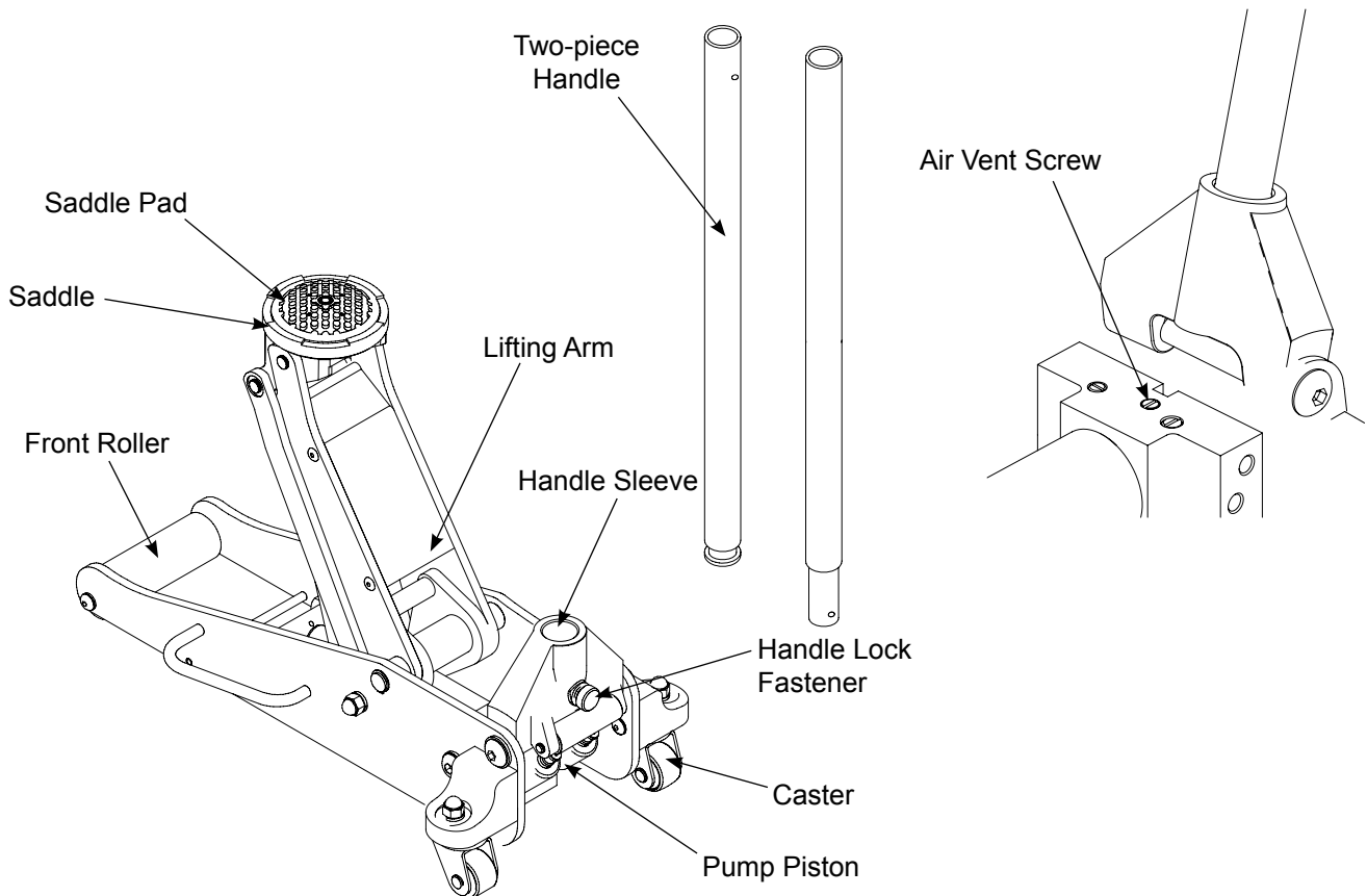
Figure 1 - Model 26022 Nomenclature
