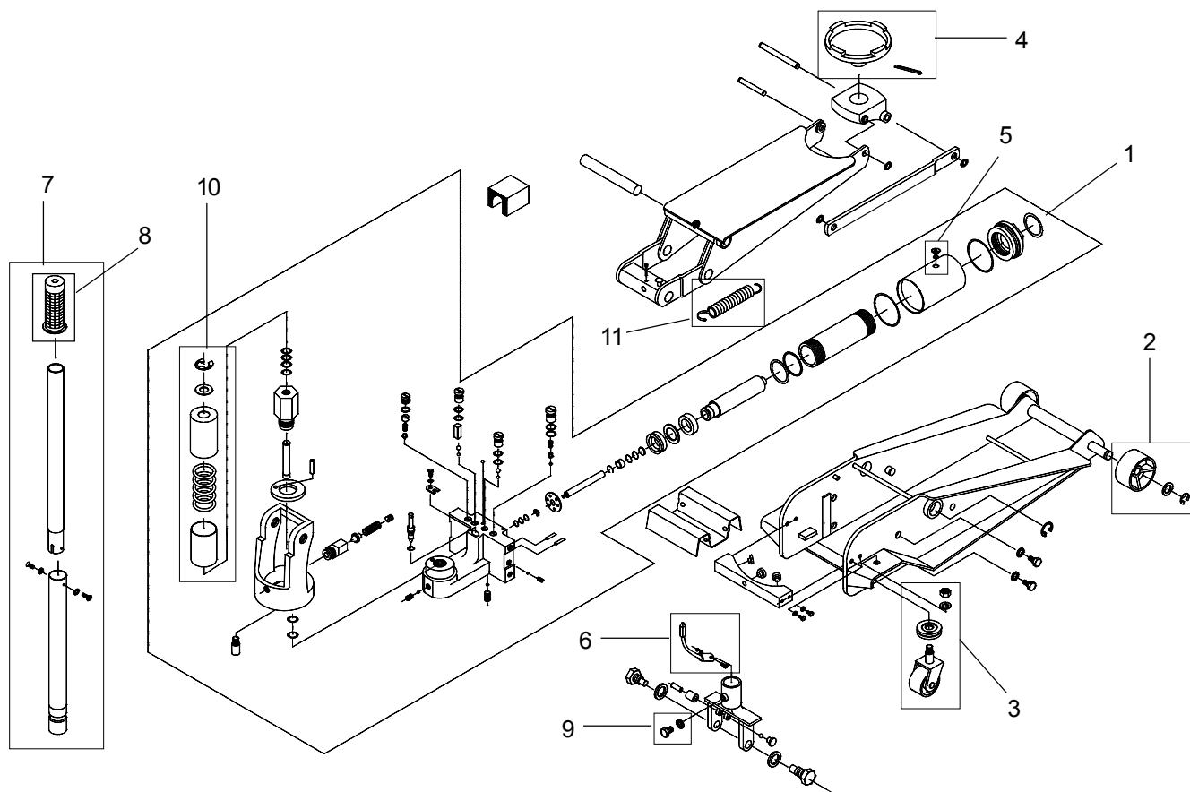
Figure 2 - Replacement Parts Illustration for Model 26025
