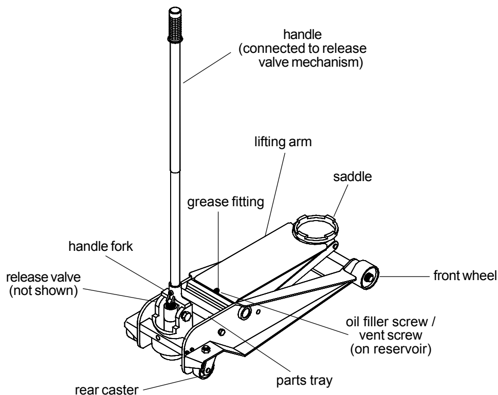
Figure 1 - Model 26025 Nomenclature
