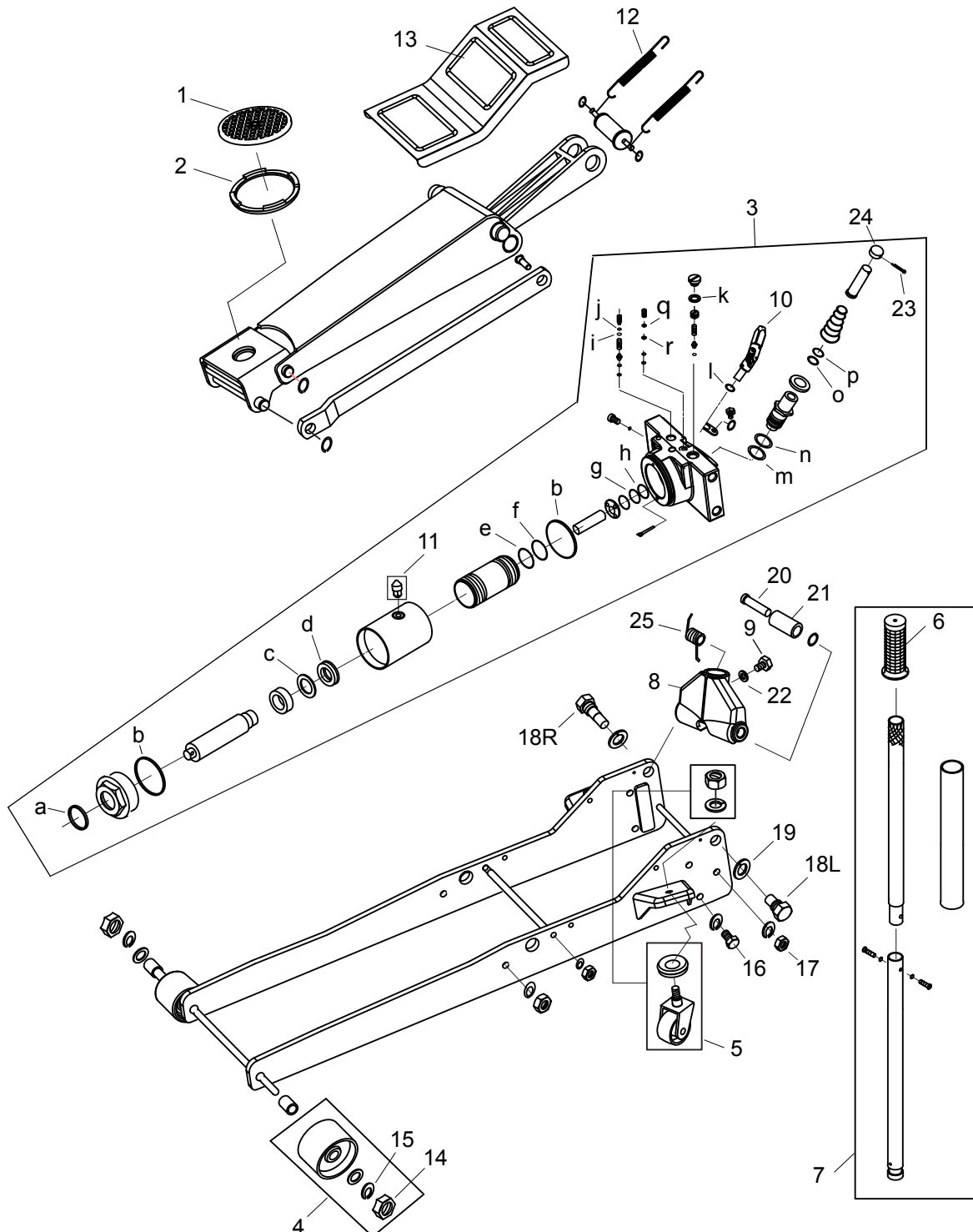
Figure 3 - Replacement Parts Illustration for Model 29023
