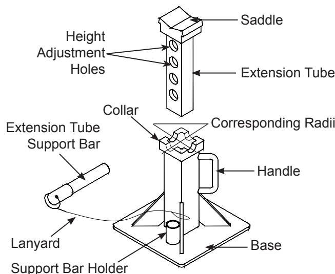
Figure 2 - Model 32225 Components
