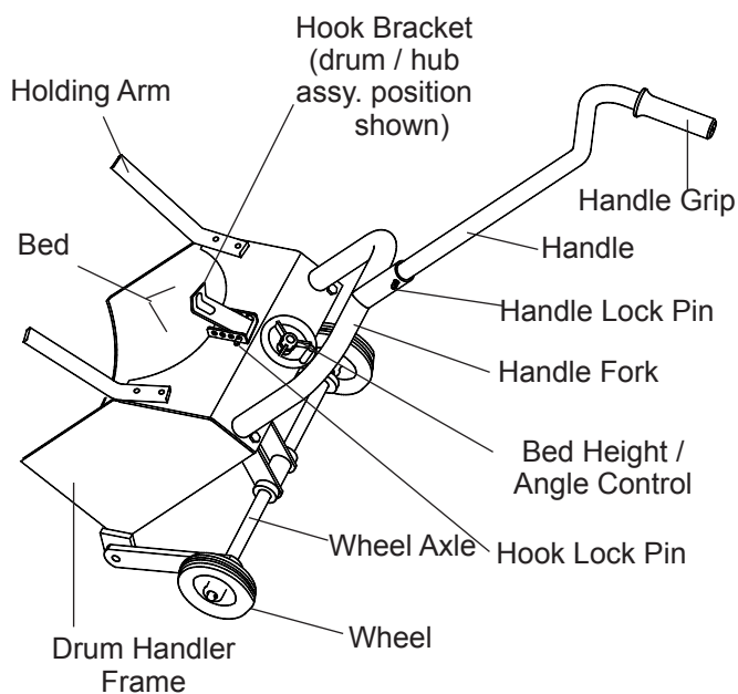
Figure 1 - Model 46000 Nomenclature
