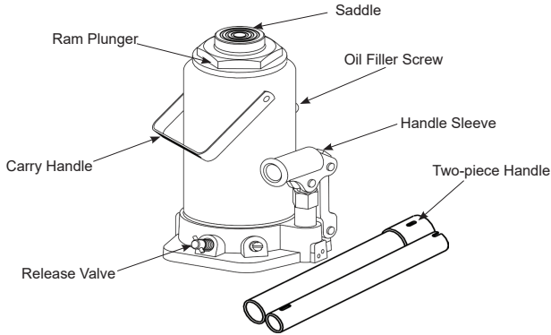
Figure 1 - Typical Bottle Jack Nomenclature
