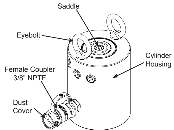
Figure 1 - Typical High Tonnage Single Acting Cylinder Components
