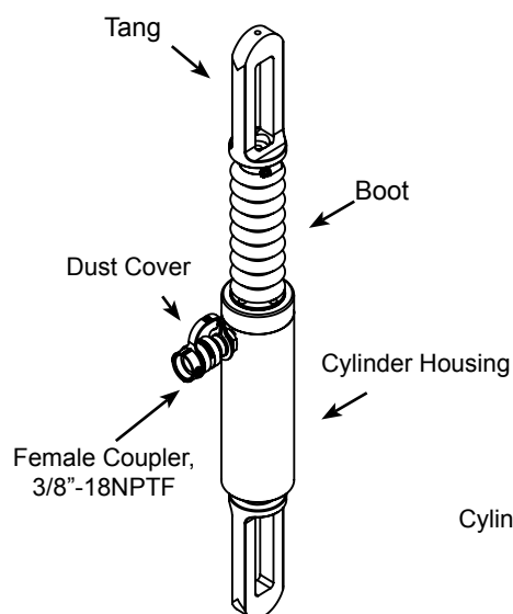
Figure 2 - HPB1006A Cylinder Components
