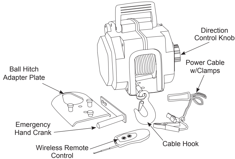
Figure 1 - Model I-9635 Nomenclature
