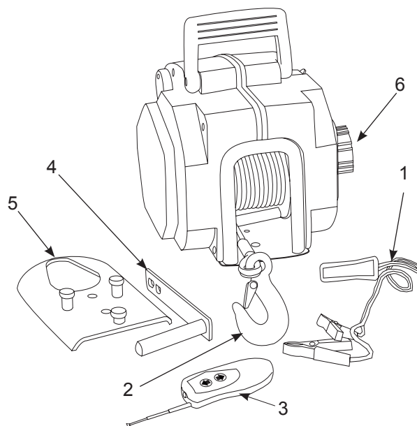
Figure 4 - I-9635 Replacement Parts
