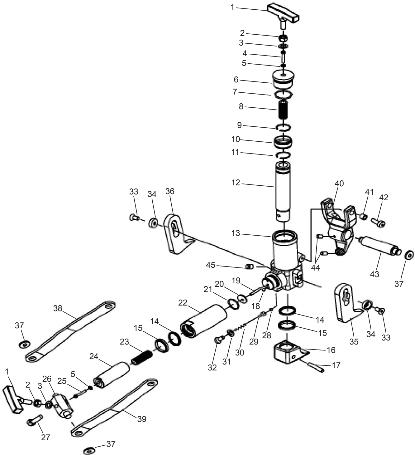
Figure 4 - Replacement Parts Illustration for Model J22910
