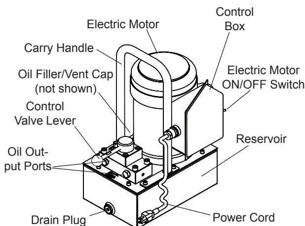
Figure 1 - Typical 4-way 3-position PEM series Electric Pump Components (PEM1002T shown)
