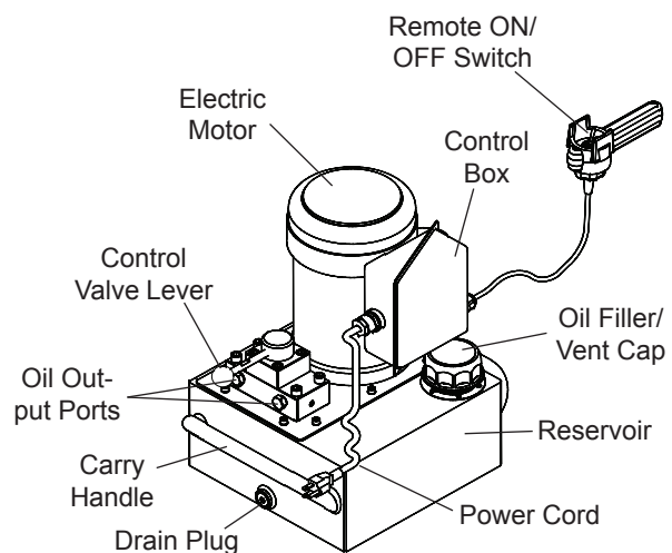
Figure 2 - Typical 4-way 3-position PEWM series Electric Pump Components (PEWM1002T shown)
